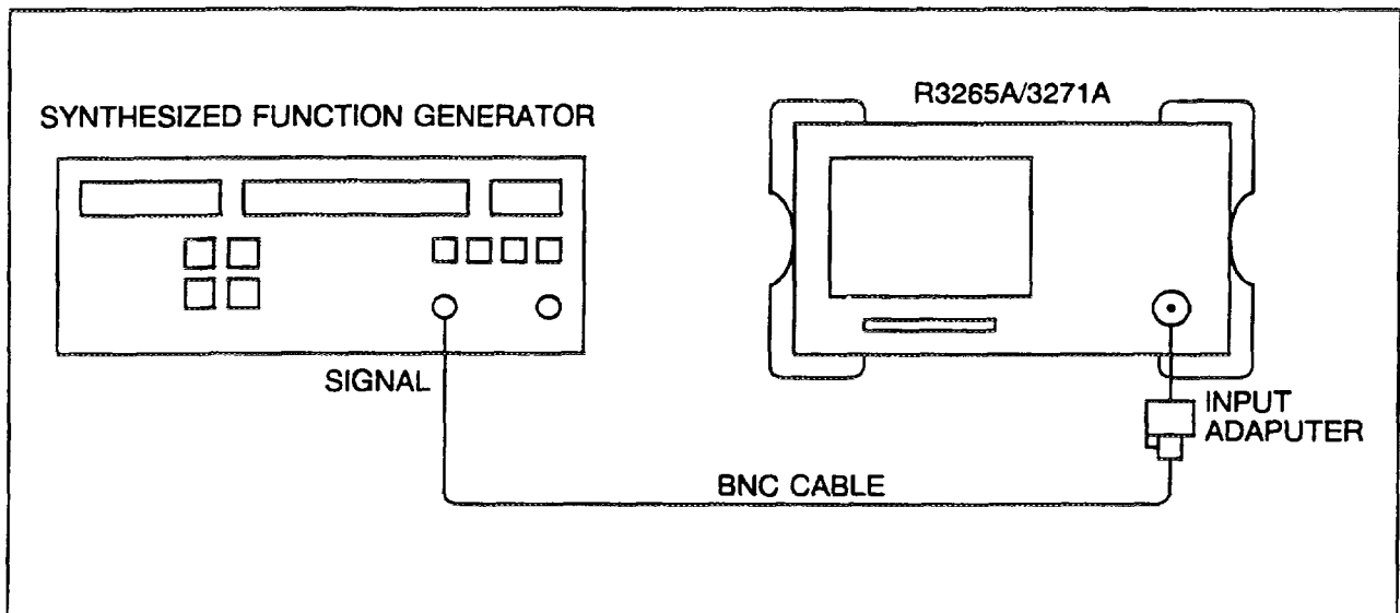
Figure 4-18 Sweep Time Accuracy Test Setup
