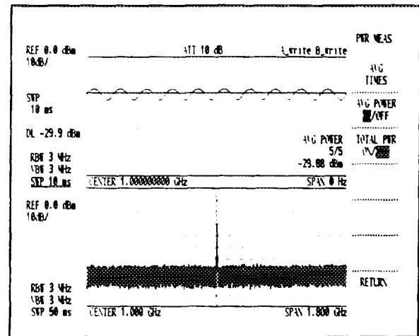
Figure 7 - 12 Measurement Screen in TIME-domain/F-domain Mode
