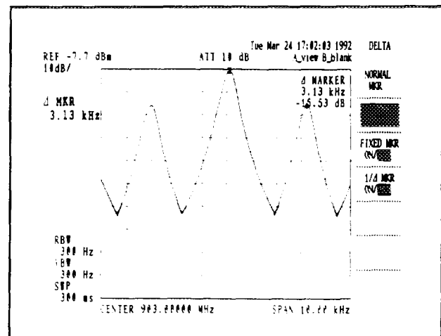
Figure 4-15 FM Signal f_{SB} and E_{SB}
