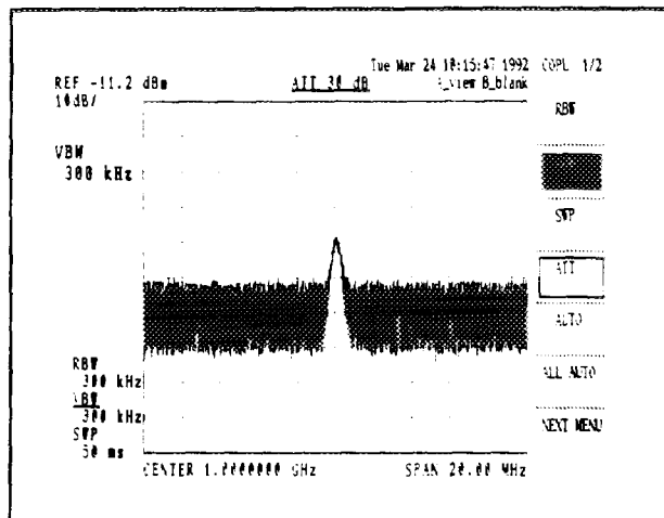
Figure 5.1-7 VBW = 300kHz
