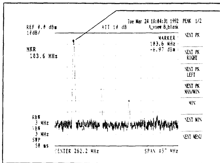
Figure 5.3-6 Peak Search Screen
