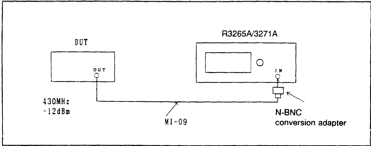
Figure 3-2 Wiring
