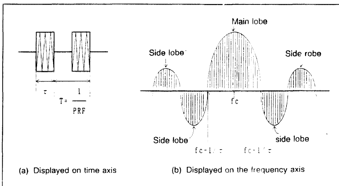
Figure 4-16 Pulse-modulated Signal
