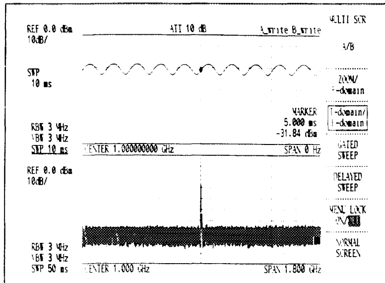
Figure 7 - 9 TIME-domain/F-domain Mode
