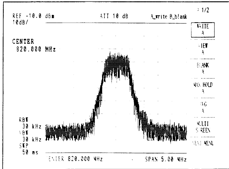
Figure 7 - 2 Full-Screen Display
