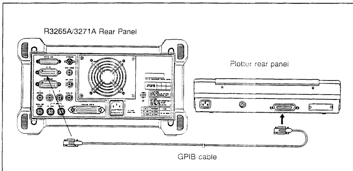
Figure 5.9-1 Plotter Connection
