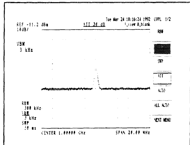
Figure 5.1-8 VBW = 3kHz
