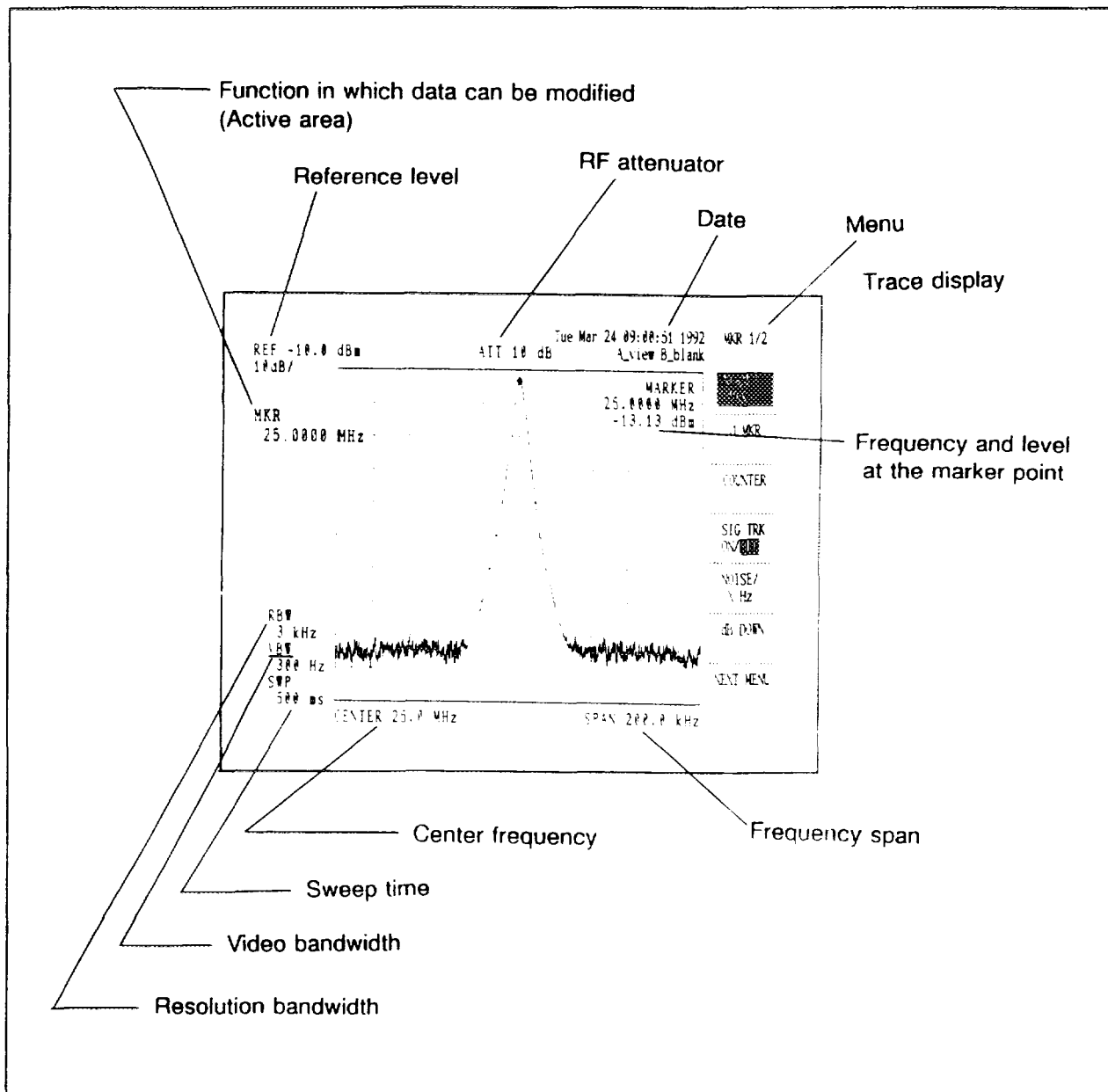
Figure 3-1 Display
