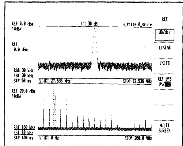
Figure 7 - 8 Measurement Screen in ZOOM/F-domain Mode
