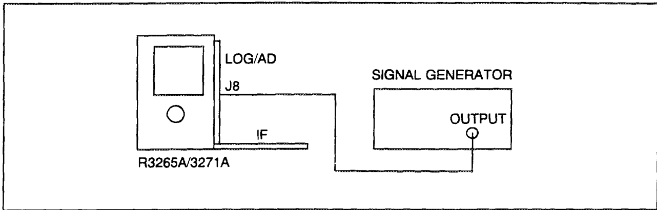
Figure 5-5 Adjustment Setup
