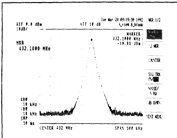
Figure 3-6 Peak Marker
